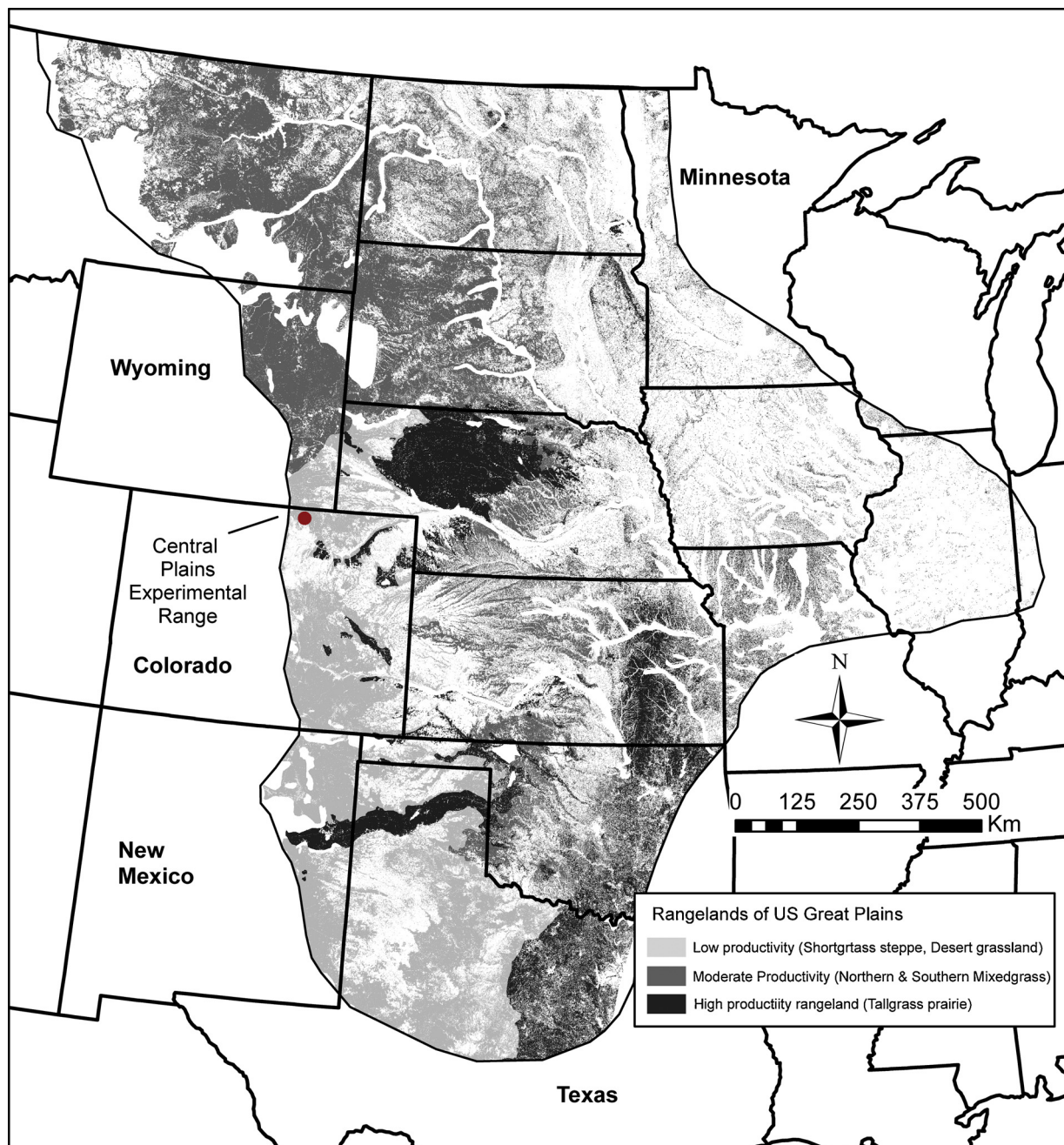
Fig. 1. Map of the United States Great Plains showing the geographic areas of the high, moderate, and low forage productivity including the location of the Central Plains Experimental Range, Nunn, Colorado, USA. Map modified from Augustine et al., ( in press ).
